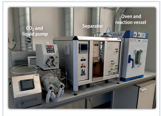
Fig. 3. The reactor at Centexbel with liquid pump, reaction chamber in the oven and a separator for separating the contamination. © Centexbel
