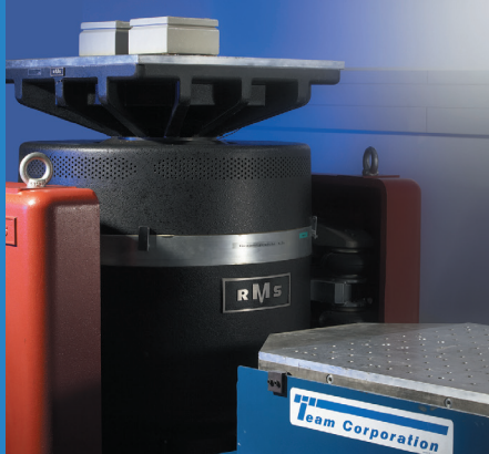
Shaker with sliding table.
