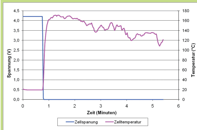
U,T-Diagramm, Nail-Penetration-Test.
